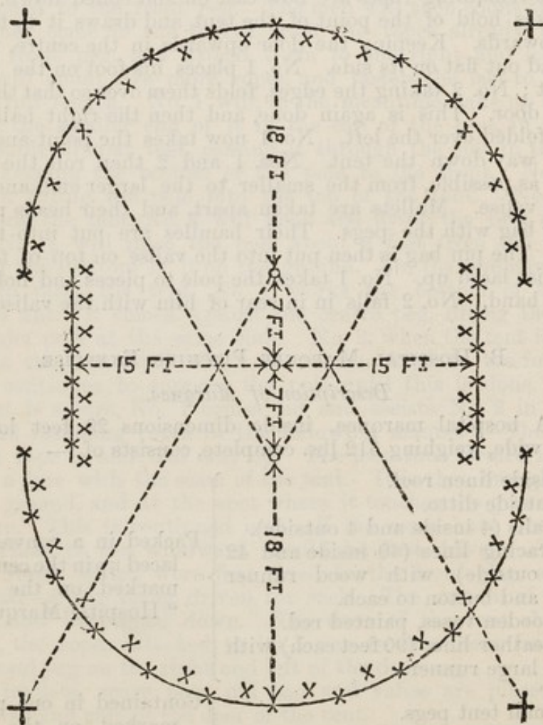
FIG. 29.—GROUND PLAN OF THE PEGS OF THE MARQUEE. (Showing direction of weather lines.)
