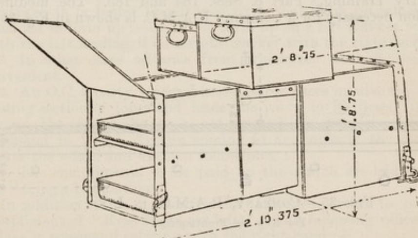
FIG. 34.—TO PUT THE STOVE TOGETHER FOR USE.
