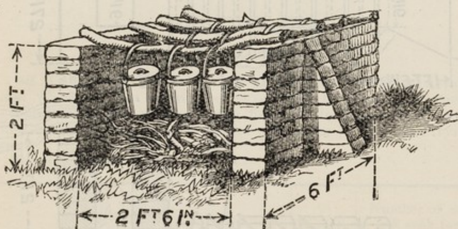
FIG. 33.—WALL KITCHEN WITH KETTLES, TO SHOW DIMENSIONS.
