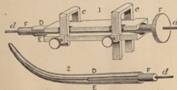
Fig. 9.—1. Handle of Perrève's dilator. c c—Clamps. d d—Conducting rod. D E—Portions of the blades. F F—Forcere on rod.
