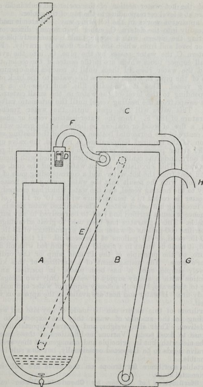
FIG. 10. FIXED TYPE OF WATER-STERILIZER.
