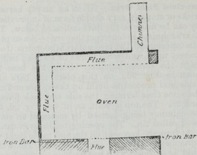
FIG. 97.—LONG SECTION. (Shaded parts indicate brick or stone.)
