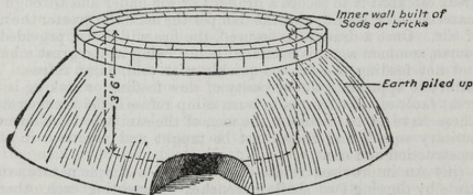
FIG. 20.—CAMP INCINERATOR—BEEHIVE.
