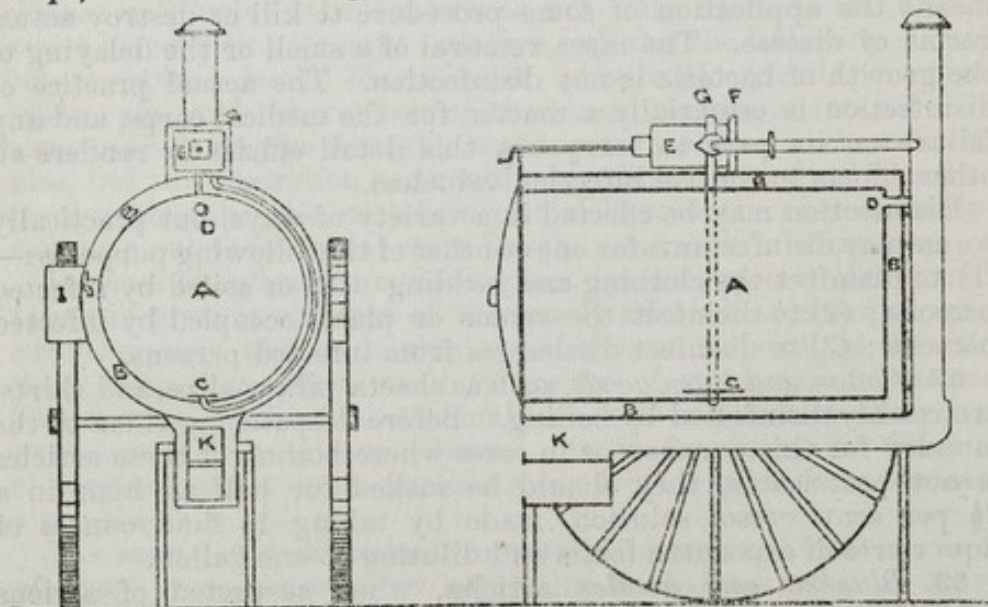
FIG. 1.—PORTABLE STEAM DISINFECTING APPARATUS (THRESH'S).
