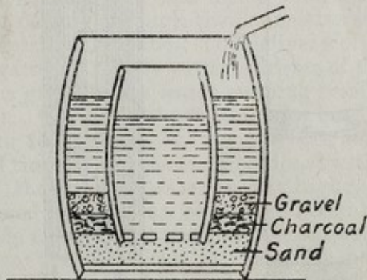
FIG. 3. IMPROVISED BARREL-FILTER.
