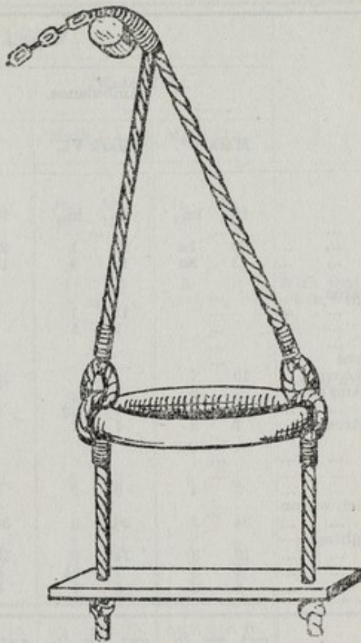
FIG. 64.—IMPROVISED LIFE-BUOY LIFT.
