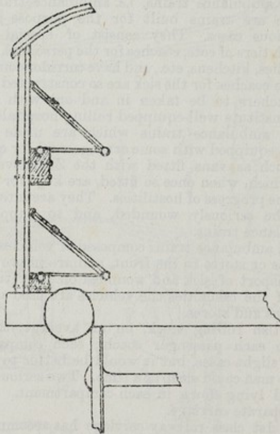
FIG. 59.—AUSTRIAN METHOD OF PREPARING RAILWAY VANS.
