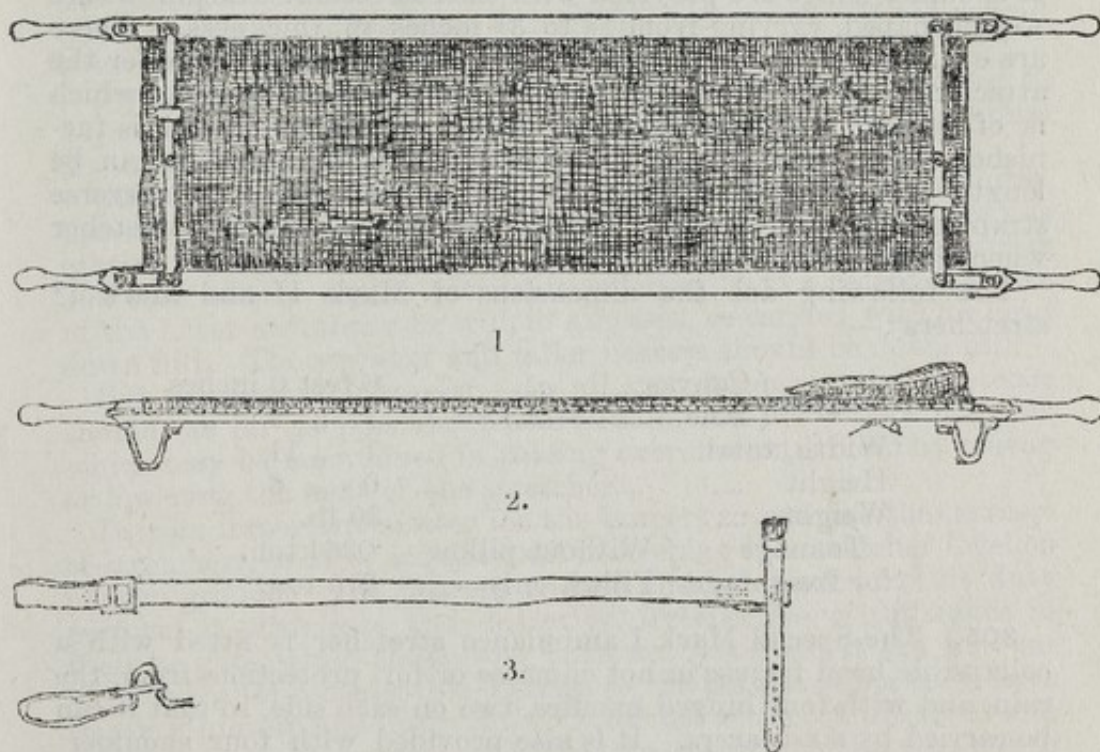
FIG. 38. AMBULANCE STRETCHERS, MARK II.
