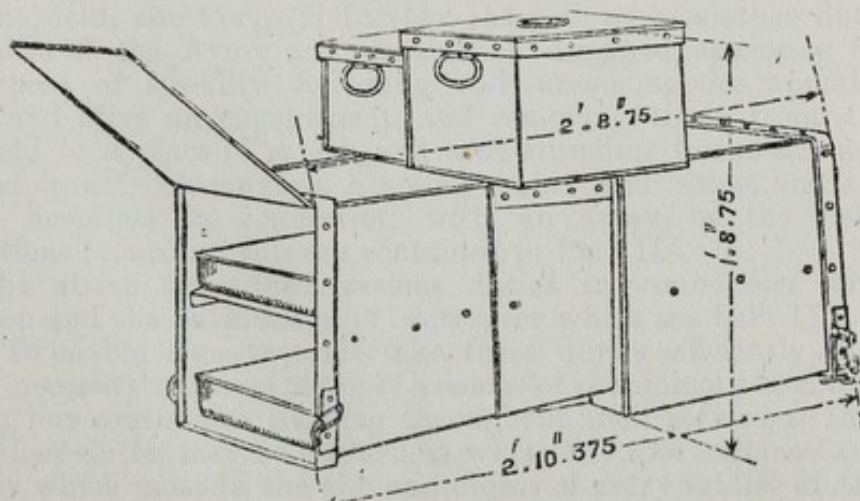
FIG. 100.—PORTABLE STOVE.
