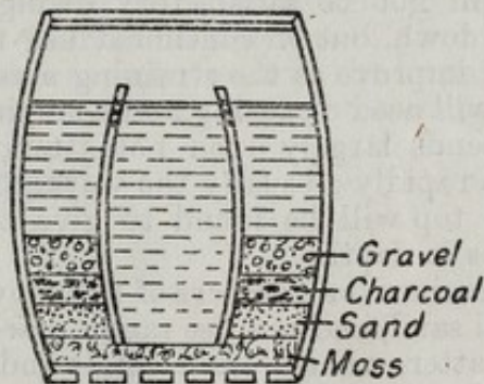
FIG. 2. IMPROVISED BARREL-FILTER.
