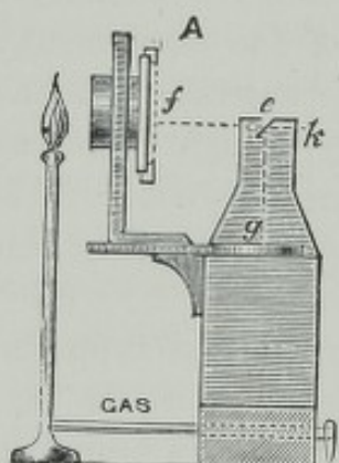
End View.
