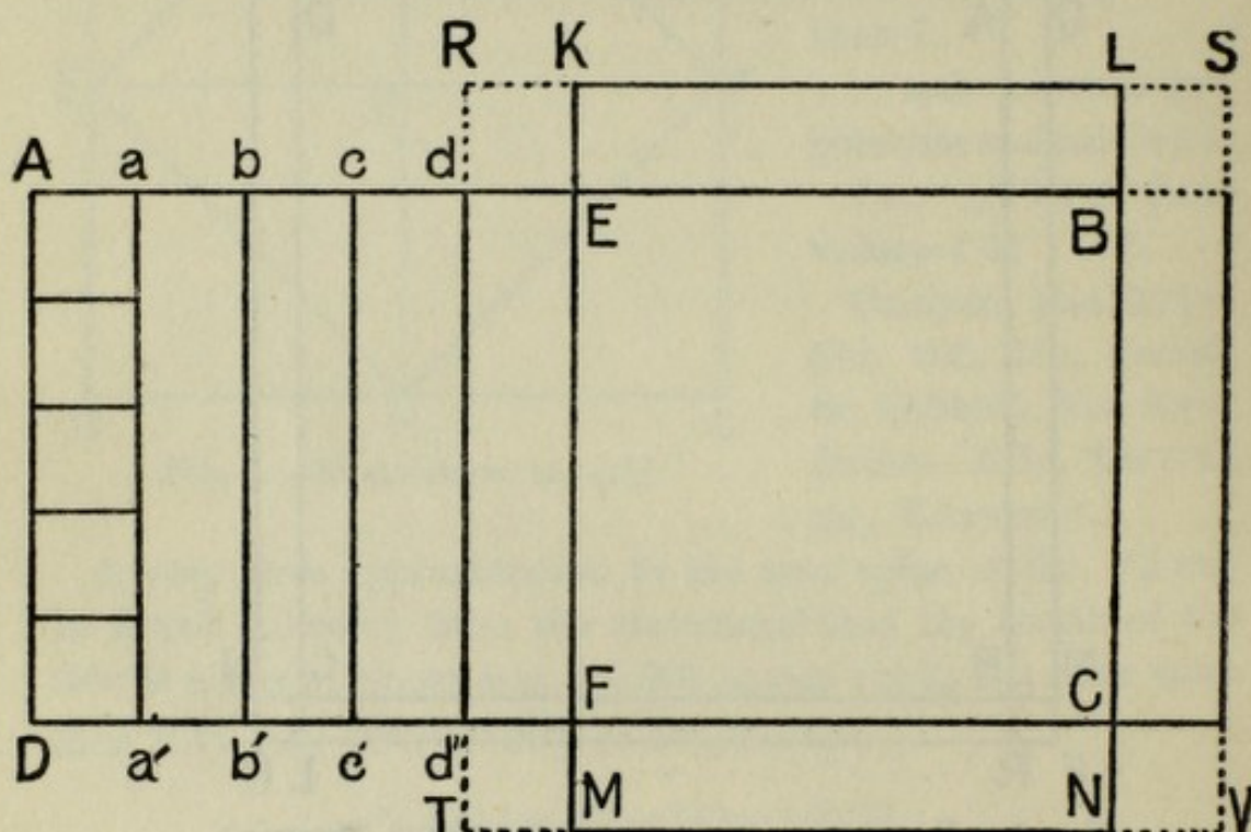
FIG. 6.—EVALUATION OF \sqrt{5000} (RASHI'S METHOD).
