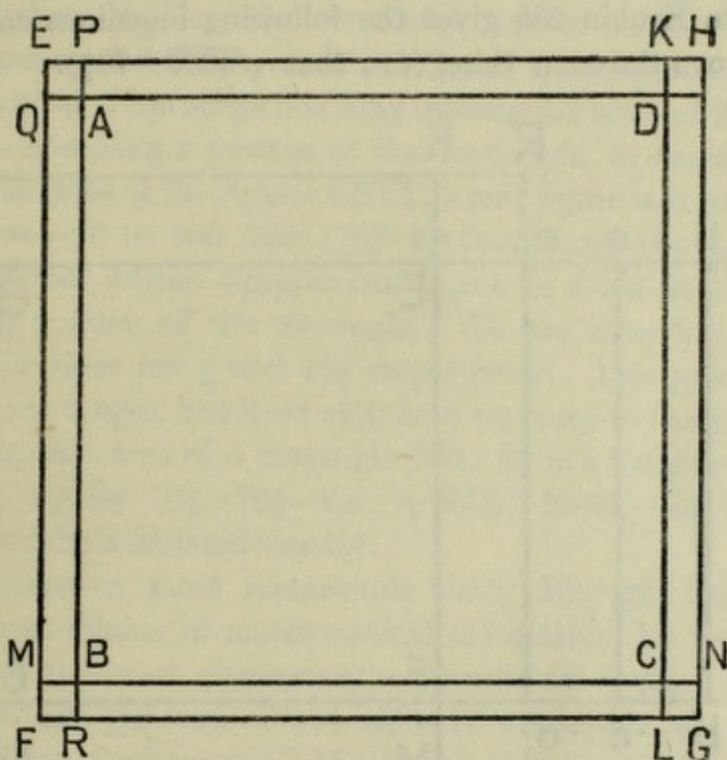
FIG. 5.—EVALUATION OF \sqrt{5000} (TALMUDIC METHOD).
