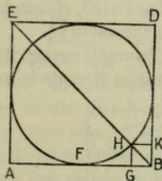
FIG. 8.—ANOTHER METHOD OF FINDING \sqrt{2} .
