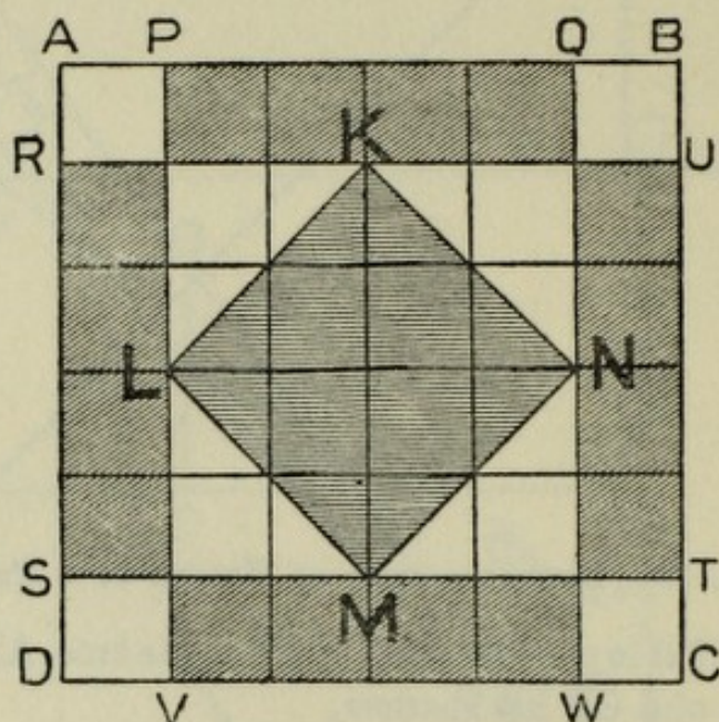
FIG. 14.—PROBLEM ON MAXIMA AND MINIMA (CASE I.).
