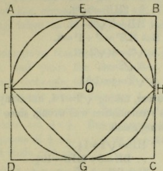
FIG. 7.—RELATION BETWEEN SQUARES AND CIRCLES.
