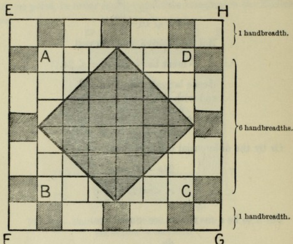
FIG. 15.—PROBLEM ON MAXIMA AND MINIMA (CASE II.).
