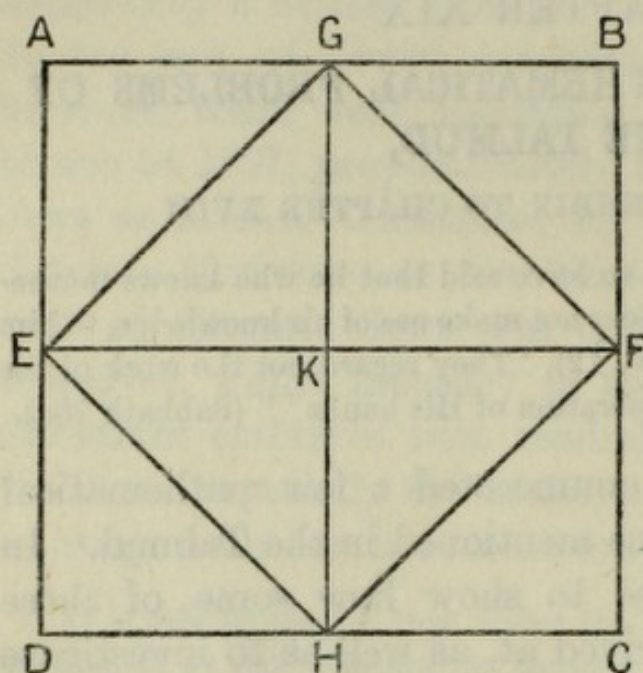
FIG. 4.—EVALUATION OF \sqrt{2} .
