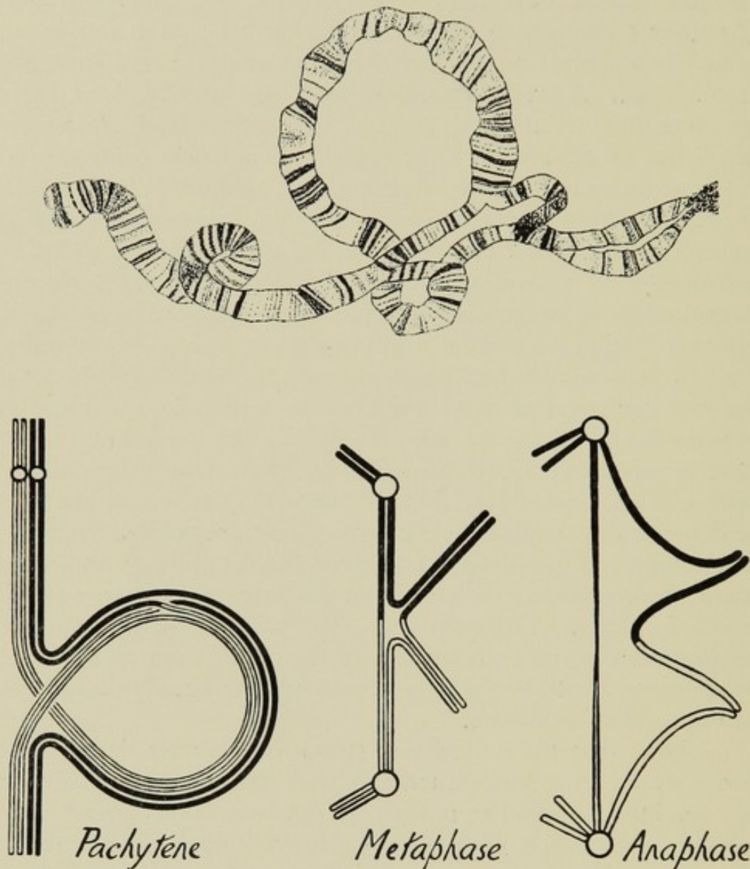
Fig. 10. Above, formation of a loop by pairing of two relatively inverted segments in the salivary gland cells of the cross of Drosophila melanogaster and D. simulans (Pätau, 1935). Below, the consequences of single crossing-over at meiosis in such an inversion hybrid with the formation of a dicentric bridge and an acentric fragment.
