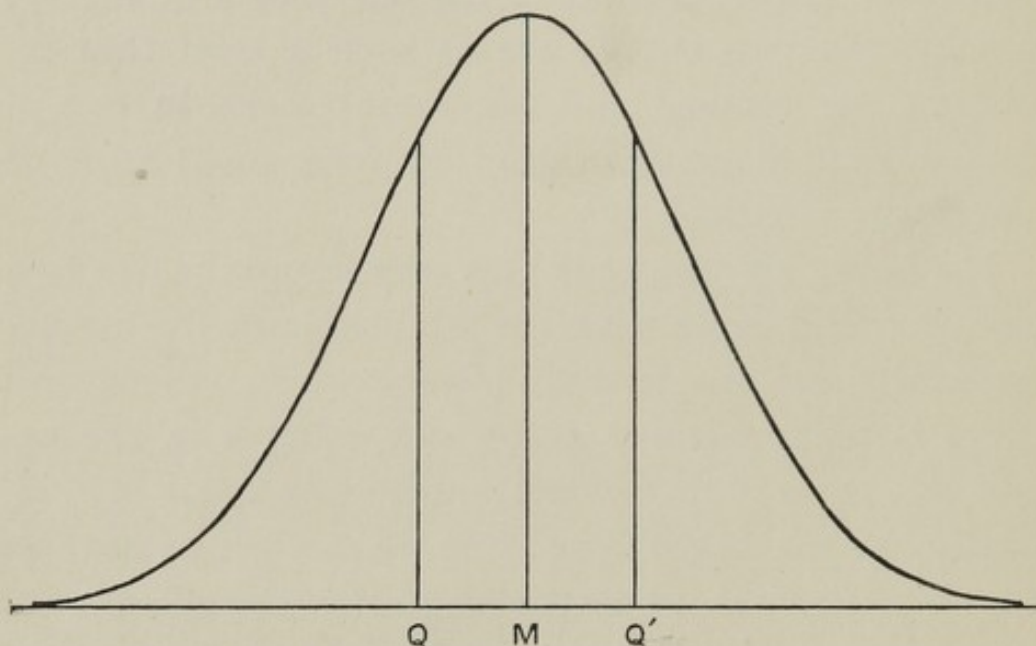
FIG. 8.—NORMAL CURVE.
